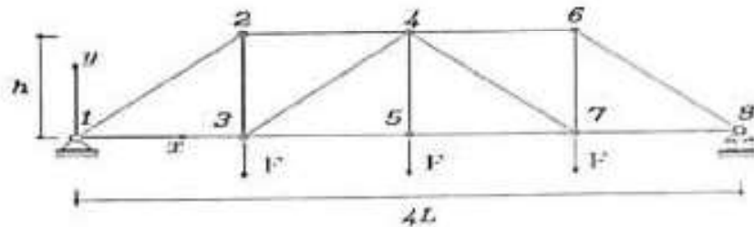
Figure 1.1: Example truss structure, constraints and loads.
