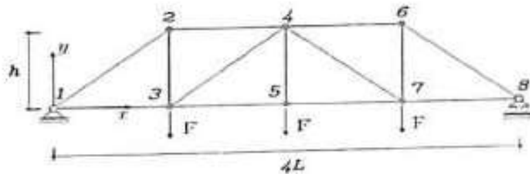
Figure 1.1: Example truss structure, constraints and loads
